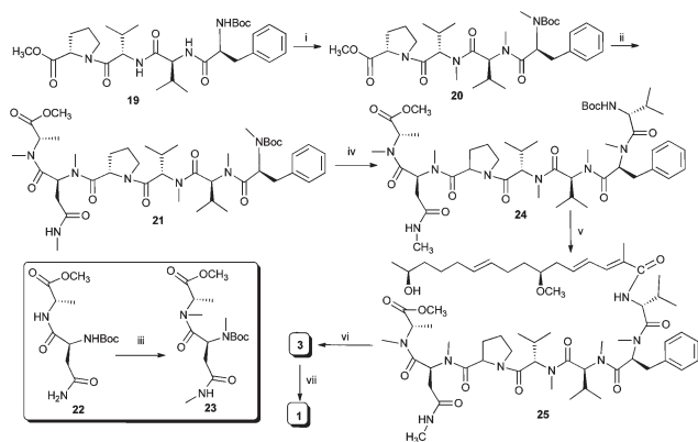
Scheme 5 Synthesis of peptide fragment and completion of the total synthesis. (i) \text{Ag}_2\text{O} , MeI, DMF, 0 °C, rt, 12 h, 72%; (ii) (a) LiOH, THF : MeOH : \text{H}_2\text{O} (3 : 1 : 1) 0 °C, rt, 1 h; (b) TFA salt of Boc-deprotected 23 , BOP-Cl, DIPEA, \text{CH}_2\text{Cl}_2 , 0 °C, rt, 12 h, 76%; (iii) \text{Ag}_2\text{O} , MeI, DMF, 0 °C, rt, 12 h, 68%; (iv) (a) TFA, \text{CH}_2\text{Cl}_2 , 0 °C, rt, 1 h; (b) Boc-D-Val-OH, BOP-Cl, DIPEA, \text{CH}_2\text{Cl}_2 , 0 °C, rt, 12 h, 79%; (v) (a) TFA, \text{CH}_2\text{Cl}_2 , 0 °C, rt, 1 h; (b) 4 , EDCI, HOBT, \text{CH}_2\text{Cl}_2 , 0 °C, rt, 15 min, then added amine from step (a), DIPEA, \text{CH}_2\text{Cl}_2 , rt, 12 h, 75%; (vi) LiOH, THF : MeOH : \text{H}_2\text{O} (3 : 1 : 1), 0 °C, rt, 1 h, 96%; (vii) MNBA, DMAP, \text{CH}_2\text{Cl}_2 , rt, 12 h, 62%.
