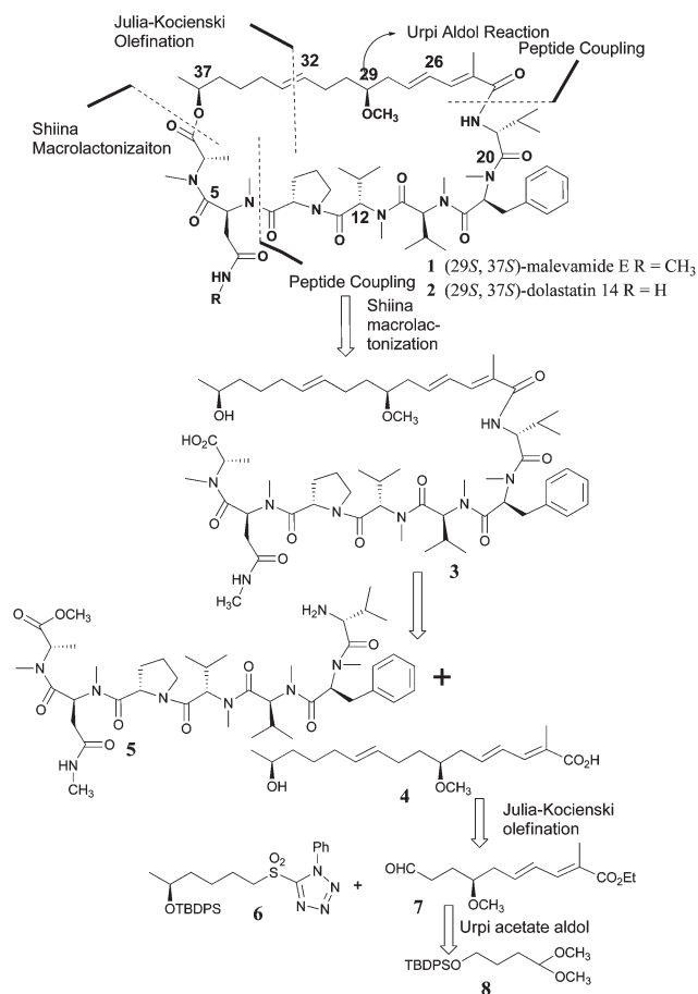
Scheme 1 Retrosynthetic analysis.
