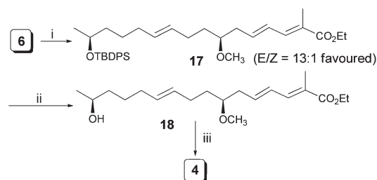
Scheme 4 Synthesis of compound 4. (i) LiHMDS, THF:HMPA, -78\text{ }^{\circ}\text{C} , aldehyde 7, -78\text{ }^{\circ}\text{C} , 3 h, 72%; (ii) TBAF:AcOH (1 : 1), \text{H}_2\text{O} , DMF, 50\text{ }^{\circ}\text{C} , 12 h, 85%; (iii) LiOH, THF:MeOH: \text{H}_2\text{O} (3 : 1 : 1), 0\text{ }^{\circ}\text{C} , rt, 1 h, 74%.
