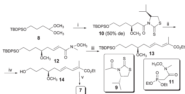
Scheme 2 Synthesis of compound 7. (i) 9, \text{TiCl}_4 , DIPEA, \text{SnCl}_4 , \text{CH}_2\text{Cl}_2 , -78\text{ }^{\circ}\text{C} , 1 h, 72%; (ii) (a) DIBAL, \text{CH}_2\text{Cl}_2 , -78\text{ }^{\circ}\text{C} , 15 min, 96%; (b) 11, NaH, THF, -40\text{ }^{\circ}\text{C} , 1 h, 78%; (iii) (a) DIBAL, \text{CH}_2\text{Cl}_2 , -78\text{ }^{\circ}\text{C} , 15 min, 97%; (b) \text{Ph}_3\text{P}=\text{C}(\text{CH}_3)\text{CO}_2\text{Et} , benzene, reflux, 3 h, 80%; (iv) TBAF, THF, 0\text{ }^{\circ}\text{C} , rt, 1 h, 85%; (v) \text{SO}_3\cdot\text{Py} , \text{Et}_3\text{N} , DCM: DMSO (2 : 1), 0\text{ }^{\circ}\text{C} , rt, 30 min, 96%.
